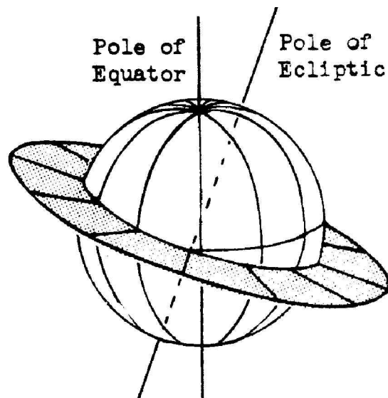
GENERAL NATURE OF THE DIVISIONS OF THE ZODIAC INTO TWELVE SIGNS OF THIRTY DEGREES EACH
